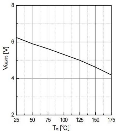
Fig 5. Typical V_{GE(th)} as a function of T_{vj} ( I_C=1mA )
