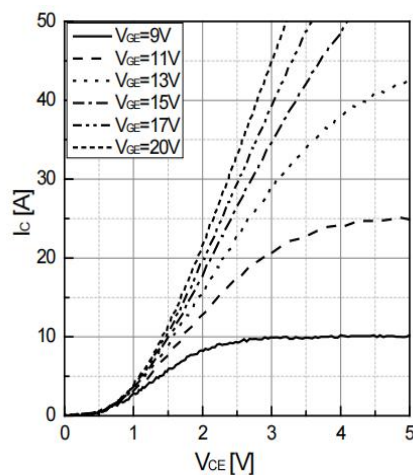
Fig 2. Typical output characteristic ( T_{vj}=175^{\circ}C )
